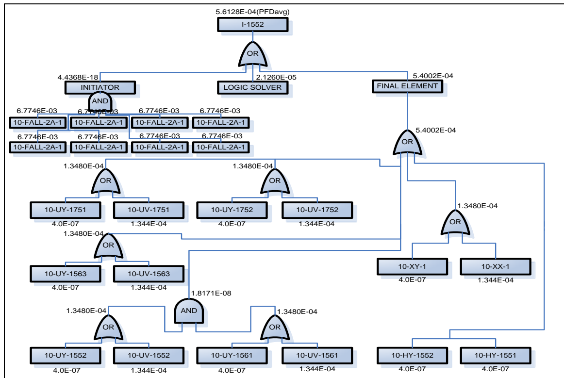
Fig. 2. Fault tree analysis for FALL-2A
